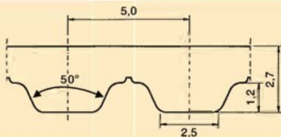
TIP AT 5 - HATVE 5 mm
